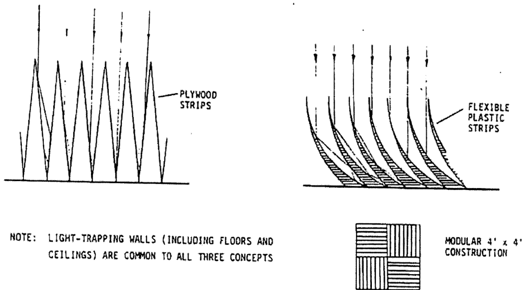
Figure 11. Light-Trapping Wall Designs.
