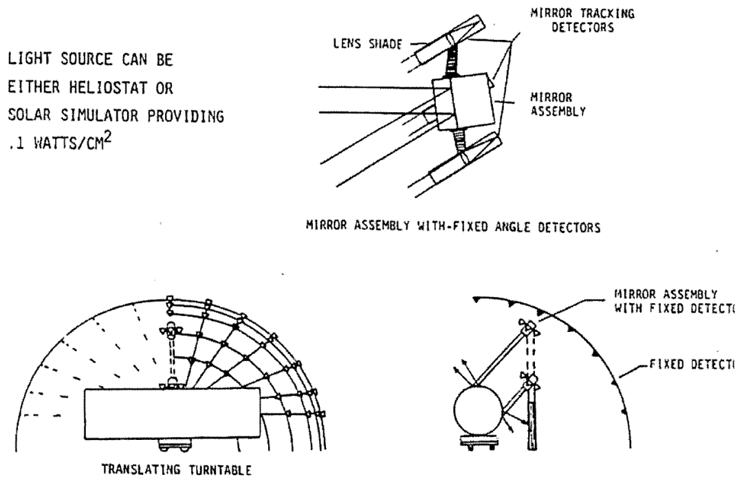
Figure 9. Concept A (Translating and Rotating Object/Movable Optics)
