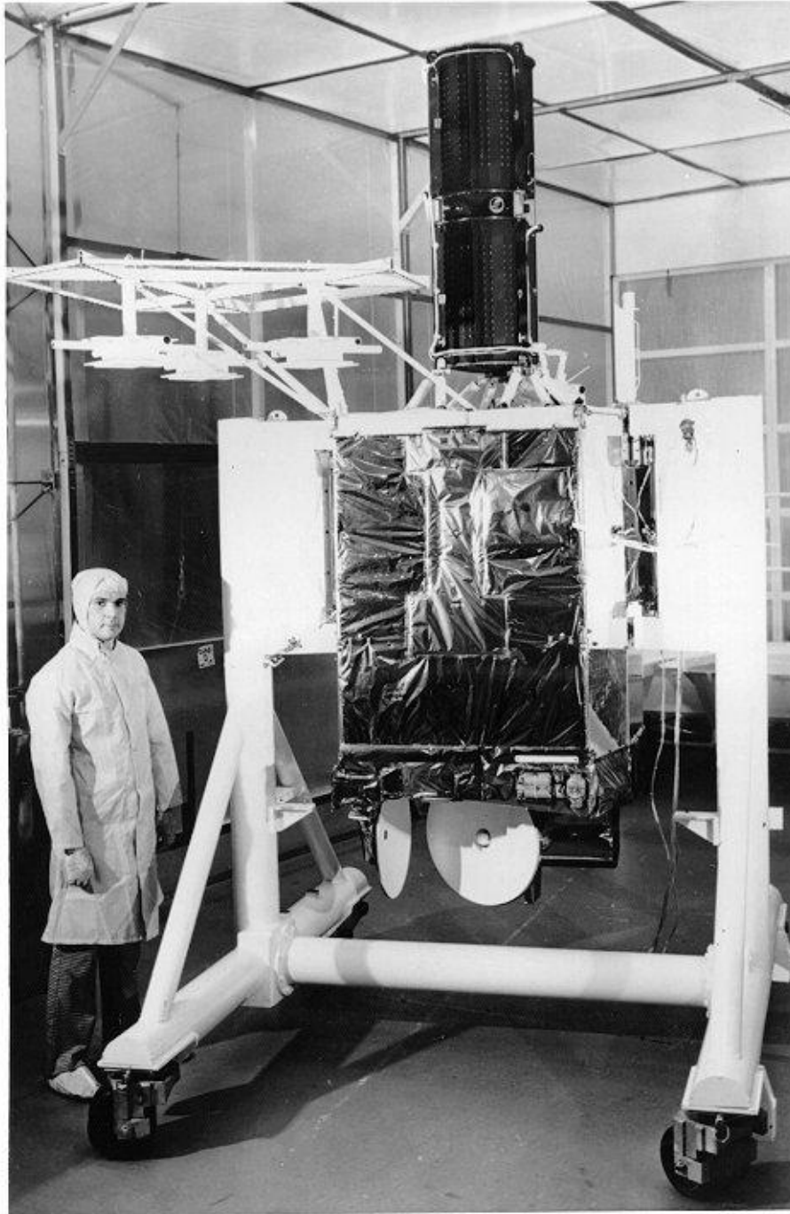
Flight Model, Lincoln Experimental Satellite
