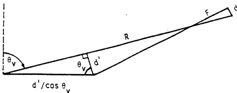
Figure 3. Projected Pixel Geometry.
