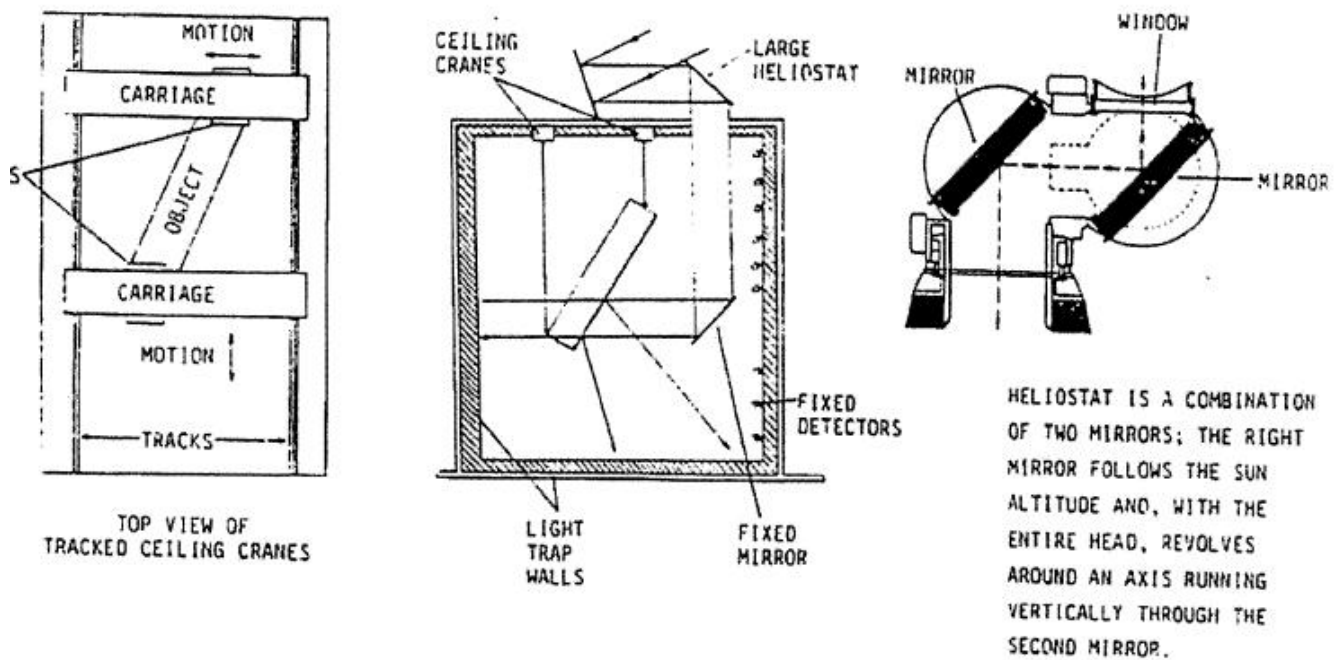
Figure 10. Concept B (Movable Object/Stationary Illumination).
