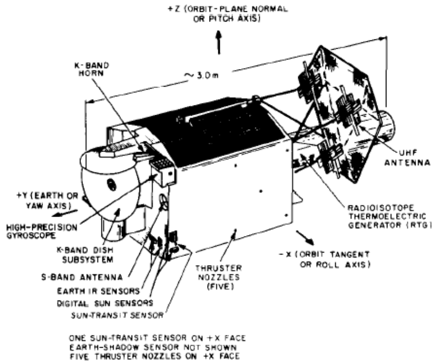
Fig. 1 Lincoln Experimental Satellites (LES) 8 and 9
