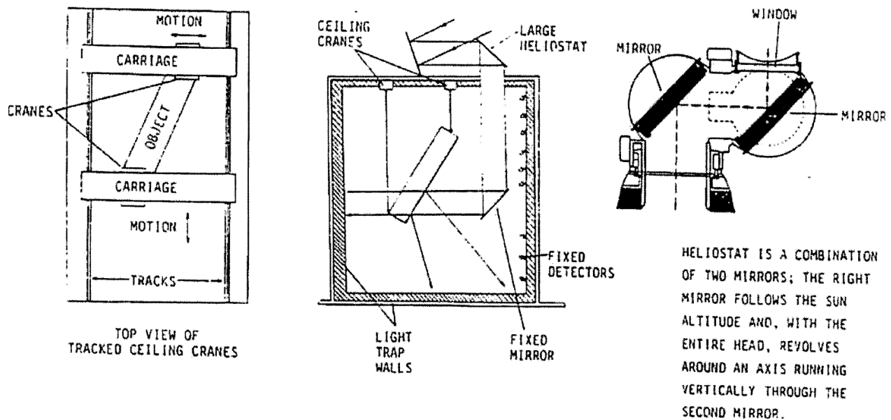
Figure 10. Concept B (Movable Object/Stationary Illumination).
